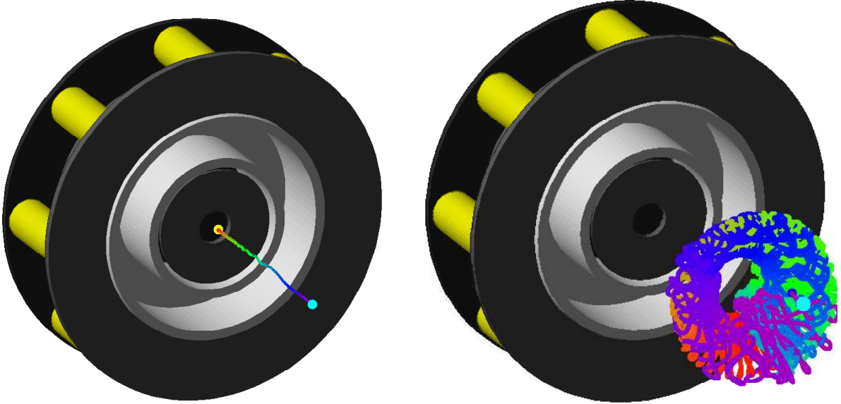
Figure 3. Two electron orbits observed out of over 10^4 in a simulation run of MCHall. Left, a typical orbit with a lifetime on the order of 10^{-7} seconds stays confined to thruster centerline after being emitted from a centrally mounted cathode (not pictured). The orbit is color-coded in time from red to violet, the yellow dot marks the sourcing point, and the blue dot marks the exit from the simulation domain. At right, an atypical secondary electron generated by an ionizing collision in the near-field is held in a confined azimuthal drift on the order of 10^{-4} seconds. This orbit is the longest-lived electron in the simulation run.
